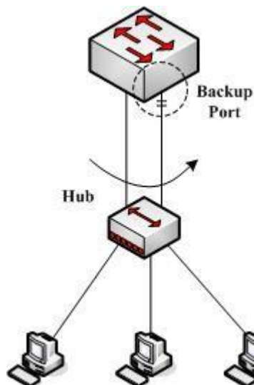
Figure 2.5 Backup port
